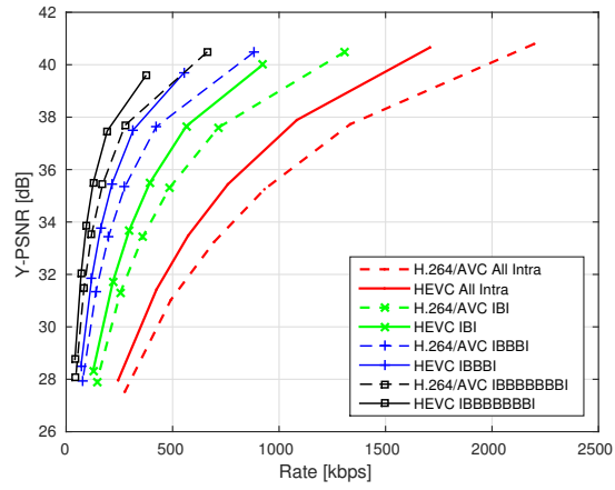
Figure 2.12: HEVC and the H.264/AVC compression performance for Hall .
