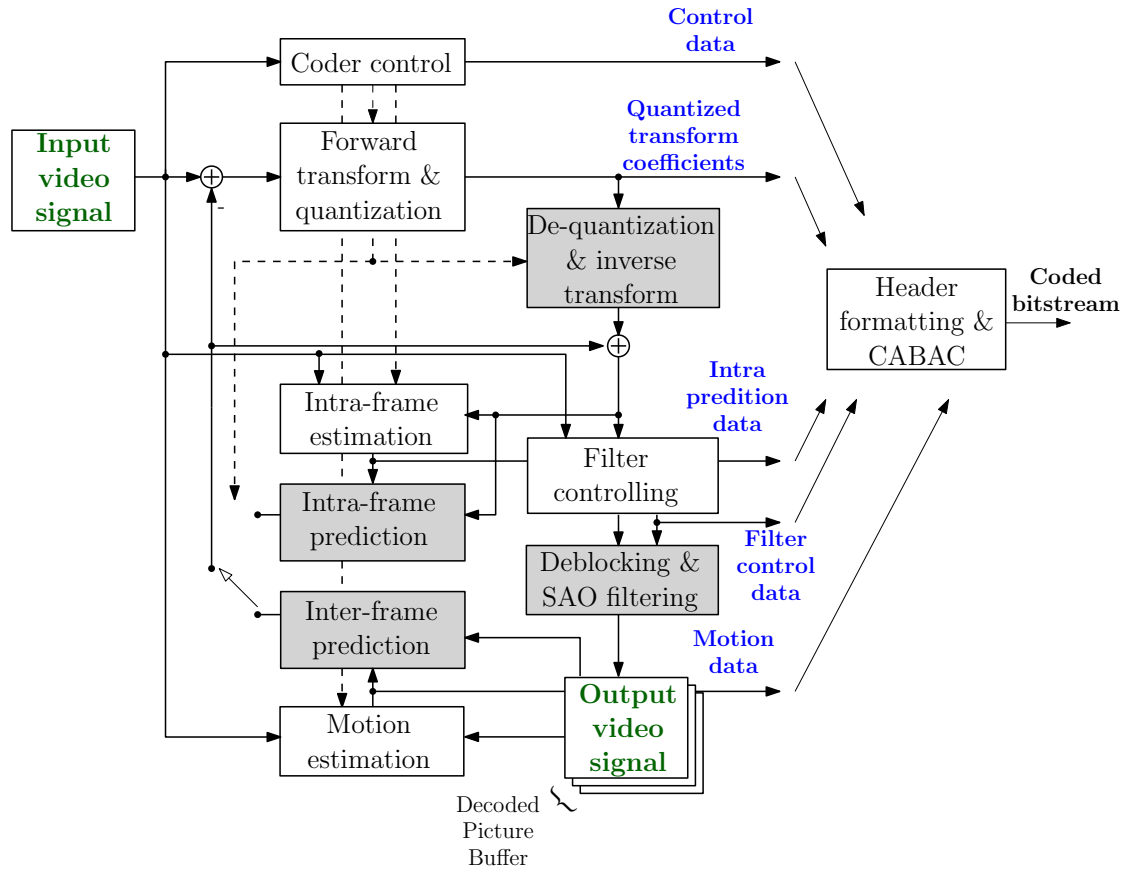
Figure 2.6: Block diagram of a typical encoder for generating an HEVC compliant bitstream. The gray blocks are the embedded decoder blocks 3 .
