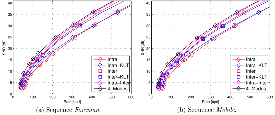
Figure 3.15: Comparative performance for SURF descriptor coding.
