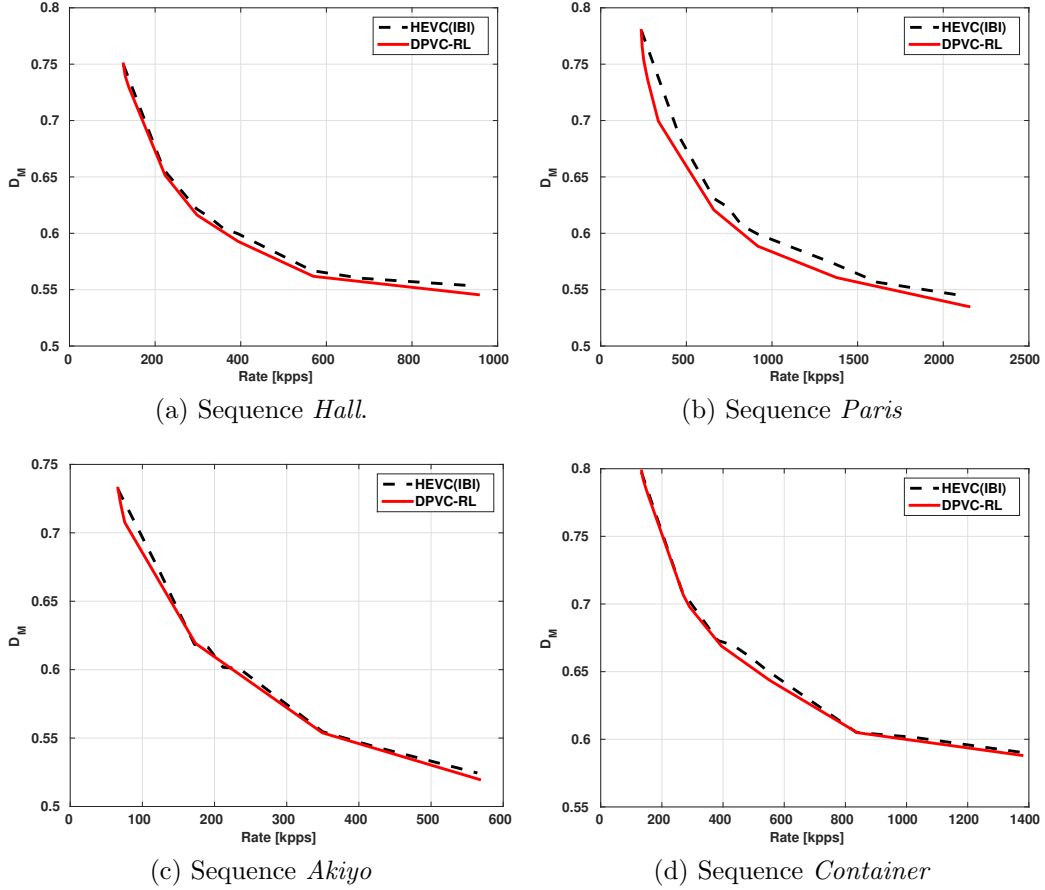
Figure 5.4: Best operational points in terms of RD_M performance obtained from the convex hull points for the tested sequences.
