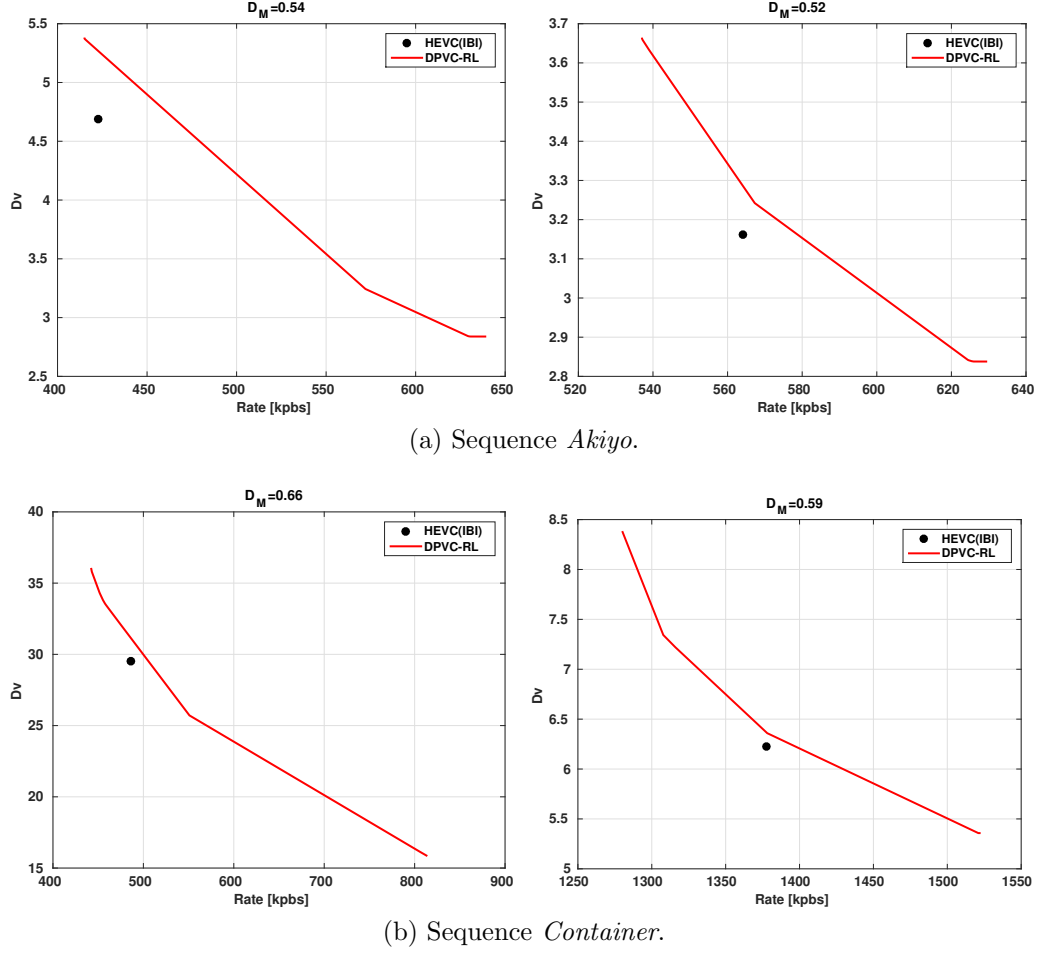
Figure 5.3: RD_V performance for two fixed descriptor matching performances for sequences: top) Akiyo and bottom) Container .
