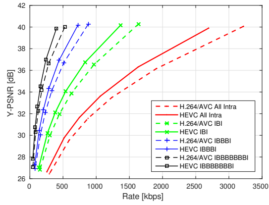
Figure 2.13: HEVC and the H.264/AVC compression performance for Container .
