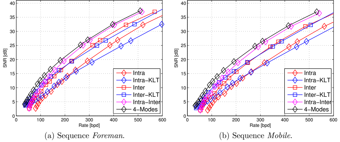
Figure 3.14: Comparative performance for SIFT descriptor coding.
