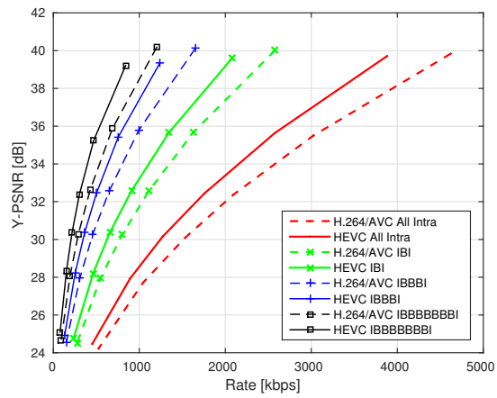
Figure 2.14: HEVC and the H.264/AVC compression performance for Paris .
