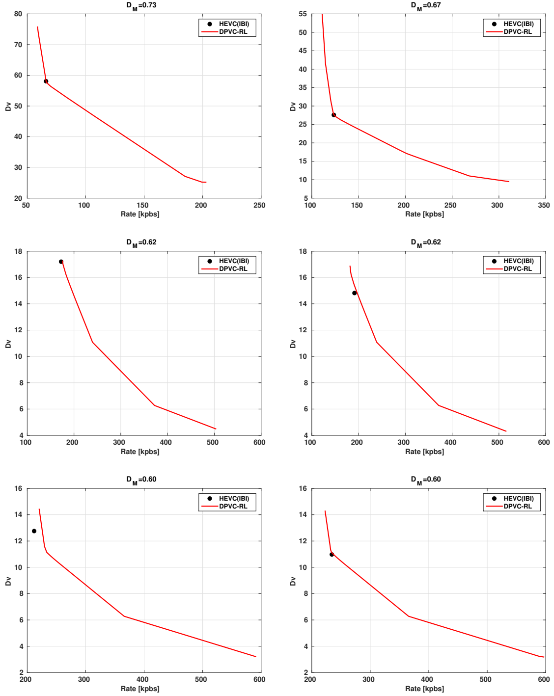
Figure D.3: RD_V performance for fixed descriptor matching performances D_M : sequence Akiyo .
