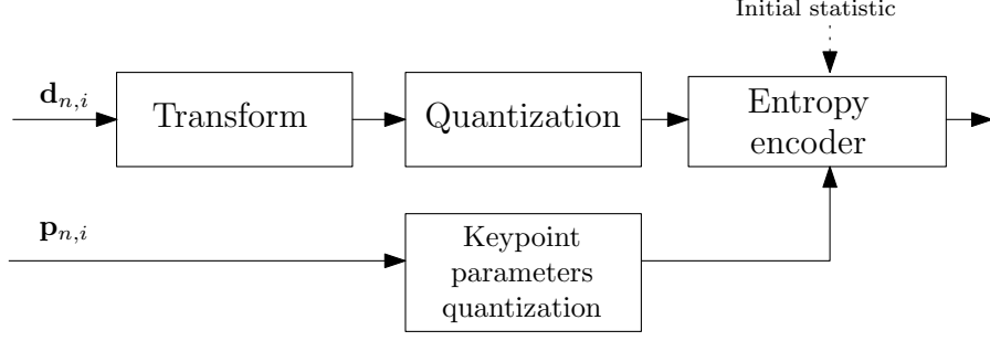
Figure 3.11: Intra coding scheme.
