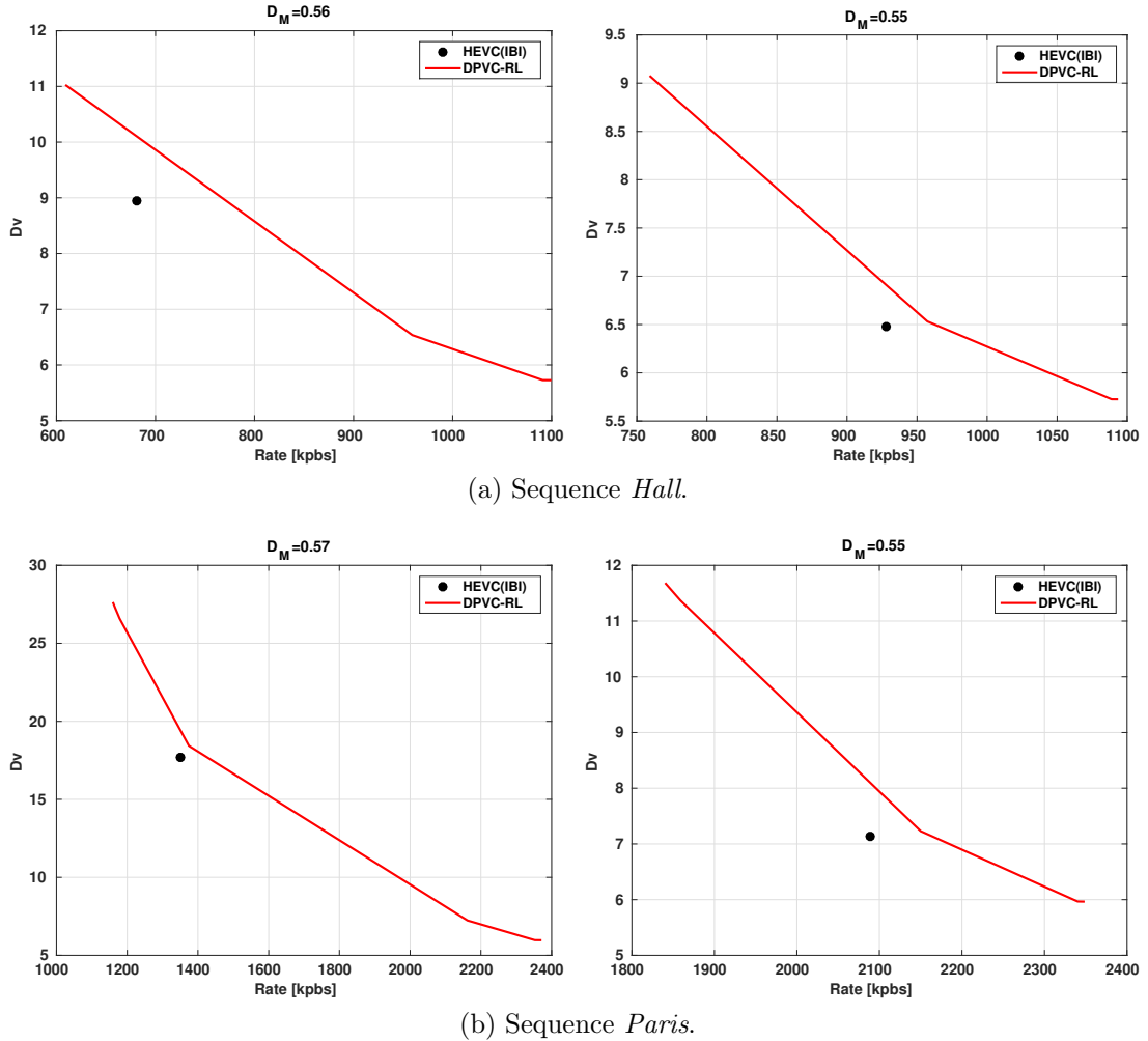
Figure 5.2: RD_V performance for two fixed descriptor matching performances for sequences: top) Hall ; and bottom) Paris .
